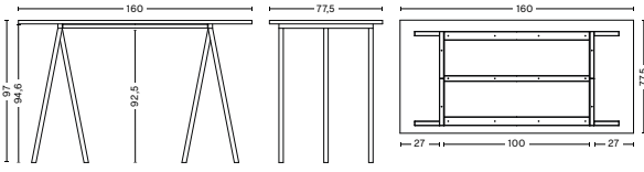
LOOP STAND TABLE HIGH WITH SUPPORT | L160 LENGTH 160 CM WIDTH 77,5 CM HEIGHT 97 CM TABLETOP THICKNESS 2,4 CM
