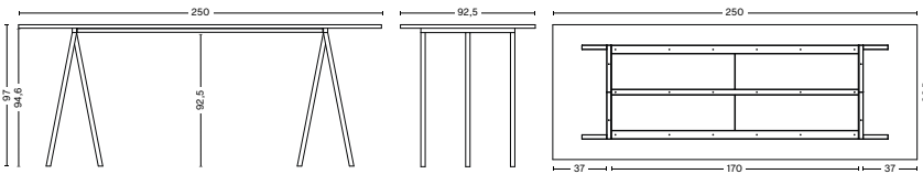
LOOP STAND TABLE HIGH WITH SUPPORT | L250 LENGTH 250 CM WIDTH 92,5 CM HEIGHT 97 CM TABLETOP THICKNESS 2,4 CM
