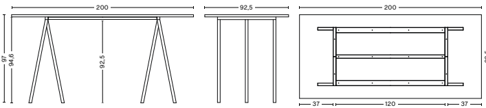
LOOP STAND TABLE HIGH WITH SUPPORT | L200 LENGTH 200 CM WIDTH 92,5 CM HEIGHT 97 CM TABLETOP THICKNESS 2,4 CM
